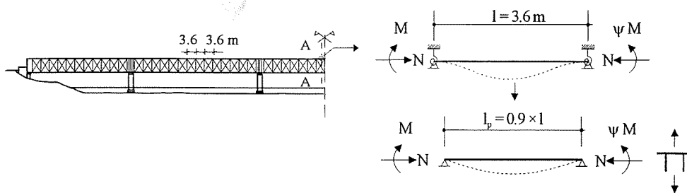
Fig.4 Simplified structural model for reliability analysis
