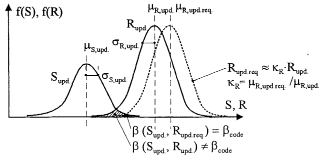
Fig. 5 Calibration of updated load and resistance models
